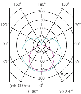
ESSENTIAL LEDtube 8W G5 840 APR
